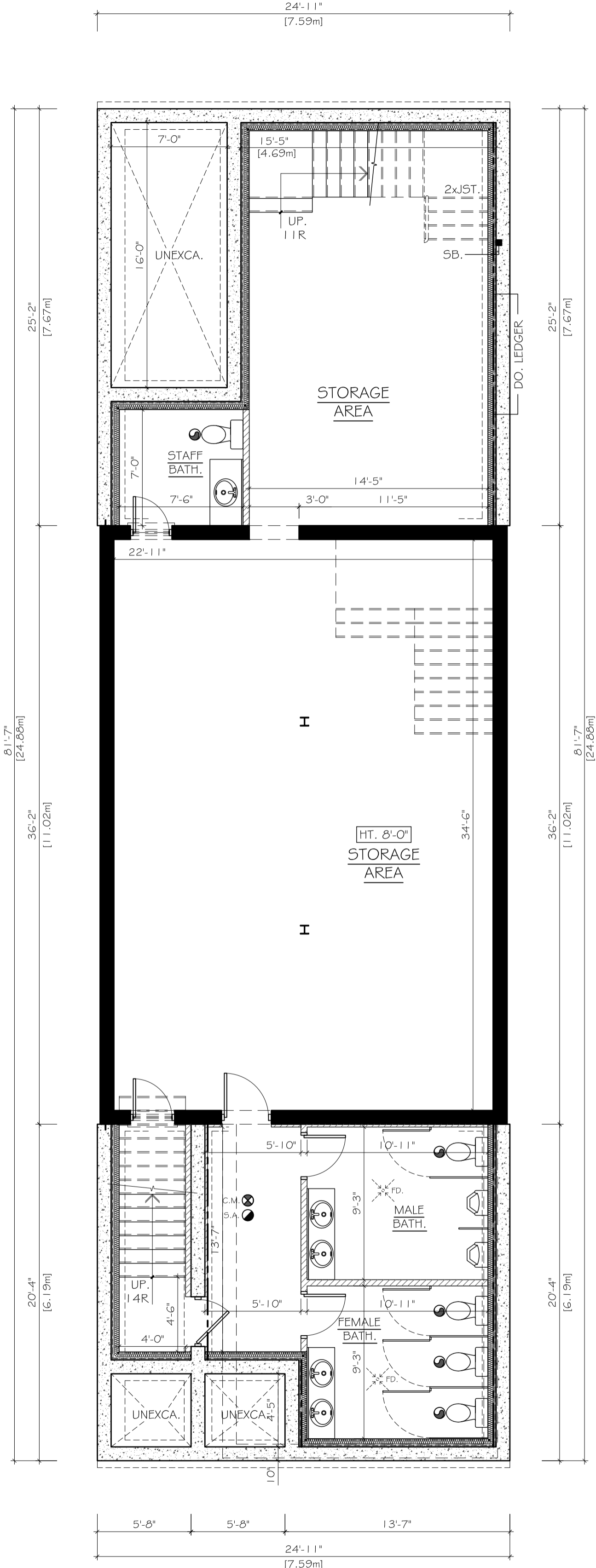
BASEMENT PLAN
