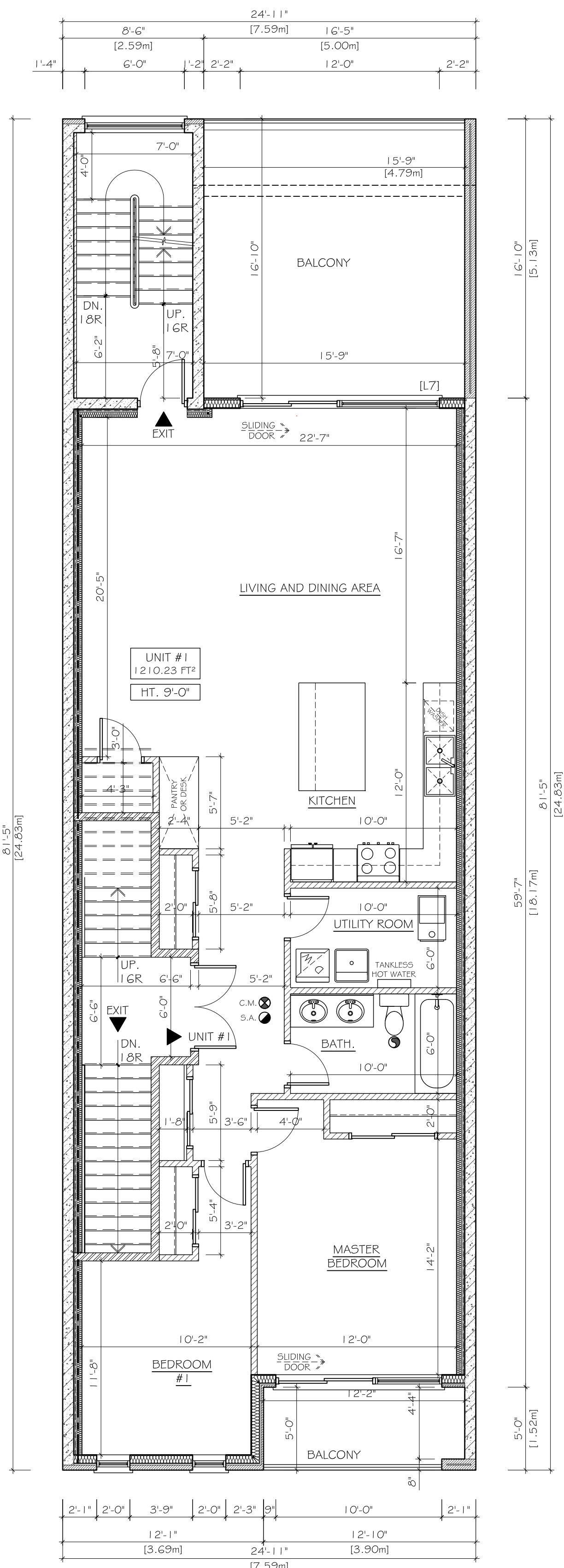
SECOND FLOOR PLAN SCALE: 3/16" = 1'-0"
