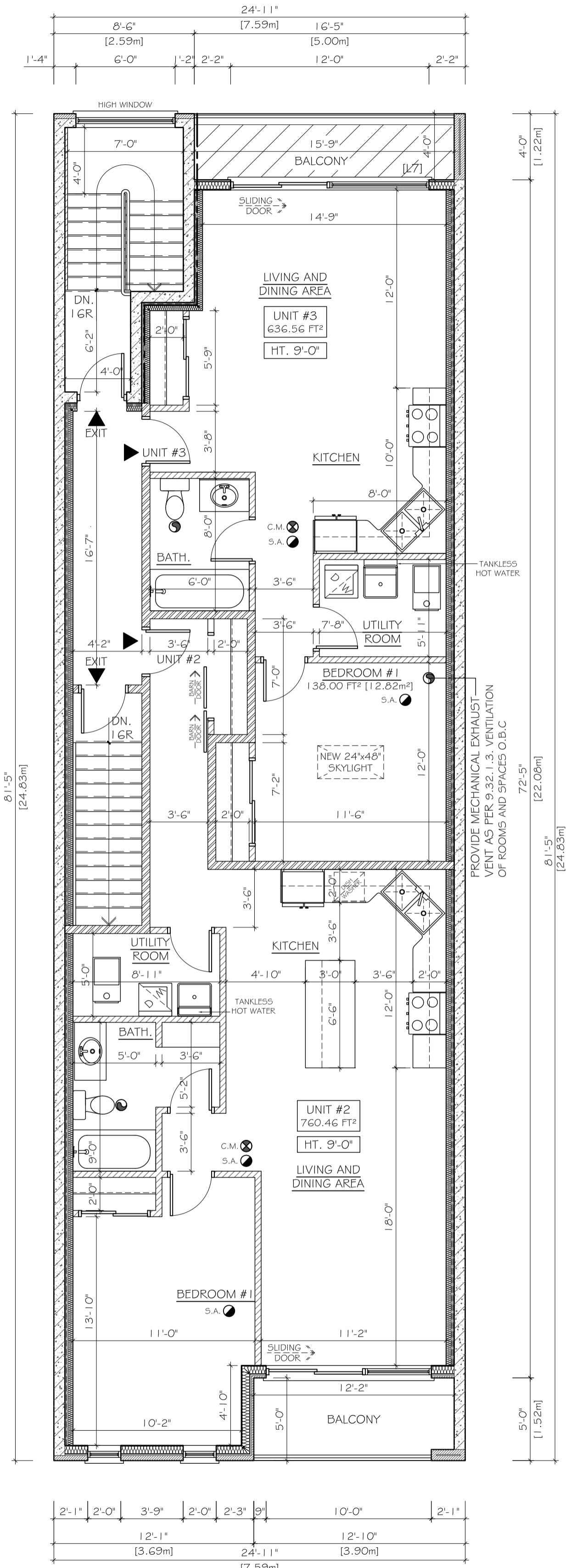
THIRD FLOOR PLAN SCALE: 3/16" = 1'-0"
